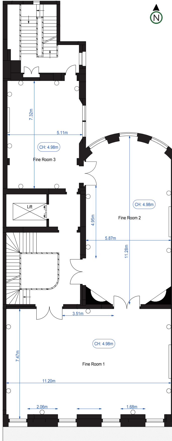
FIRST FLOOR
